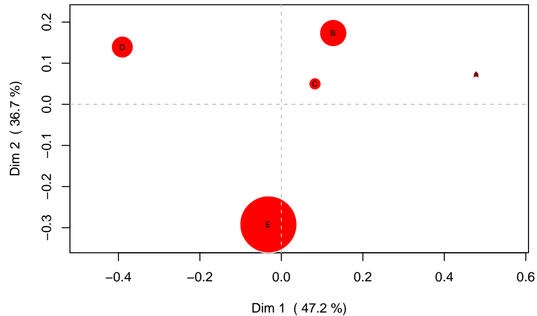
CA cols scatterplot: points proportional to the contrib. to Dim 2
