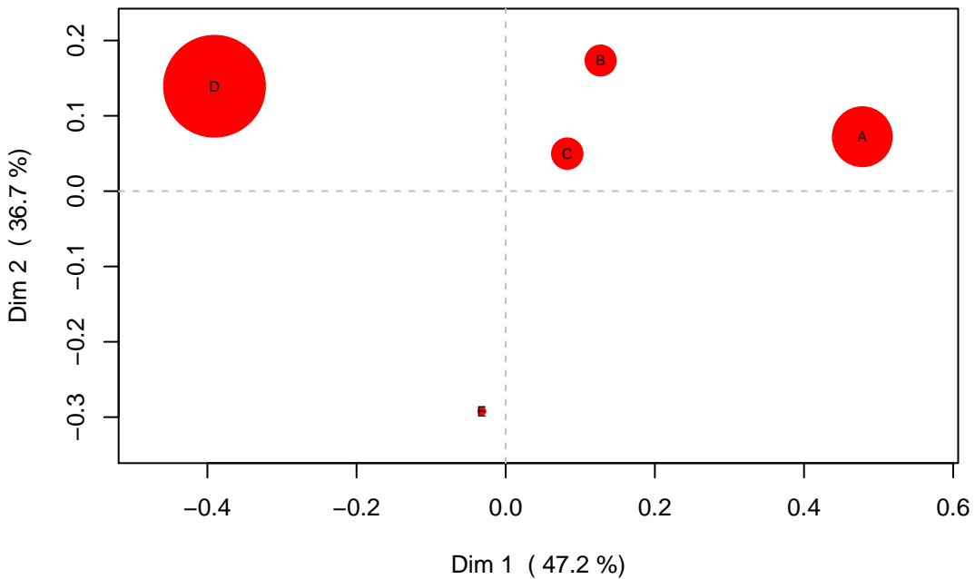
CA cols scatterplot: points proportional to the contrib. to Dim 1
