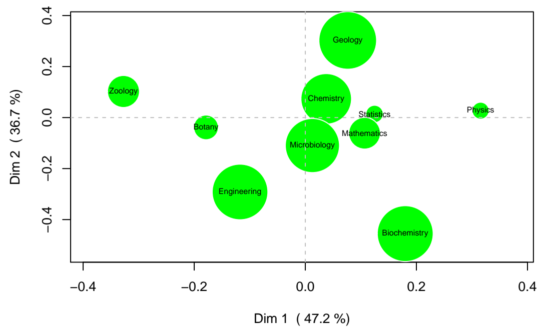
CA rows scatterplot: points proportional to the correl. with Dim 2
